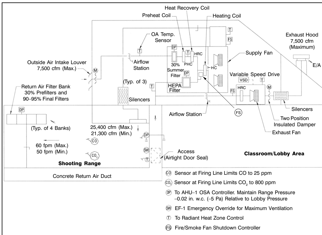
Figure 1: Firing range dilution ventilation schematic for Hunter Education Indoor Shooting Range.
